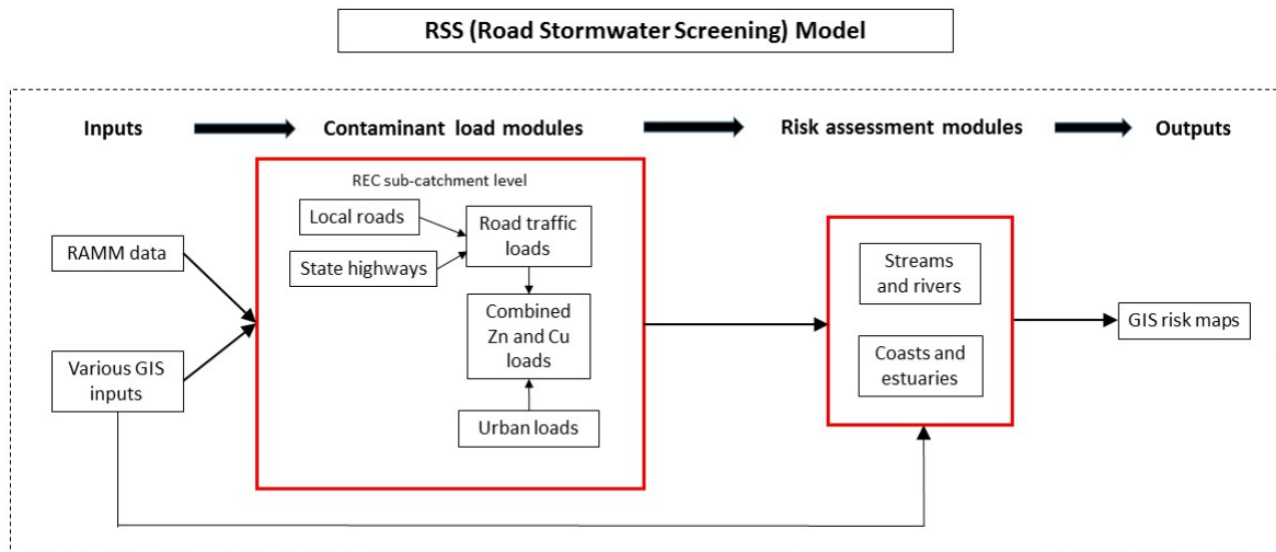
Figure 1: Schematic of RSS model
