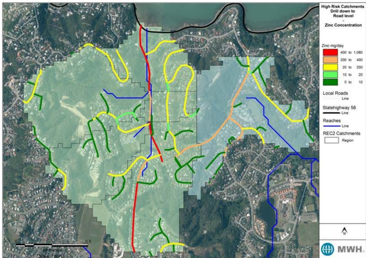
Figure 9 Example 'drill down' to identify zinc loads by road in a 'highest' risk sub-catchment
