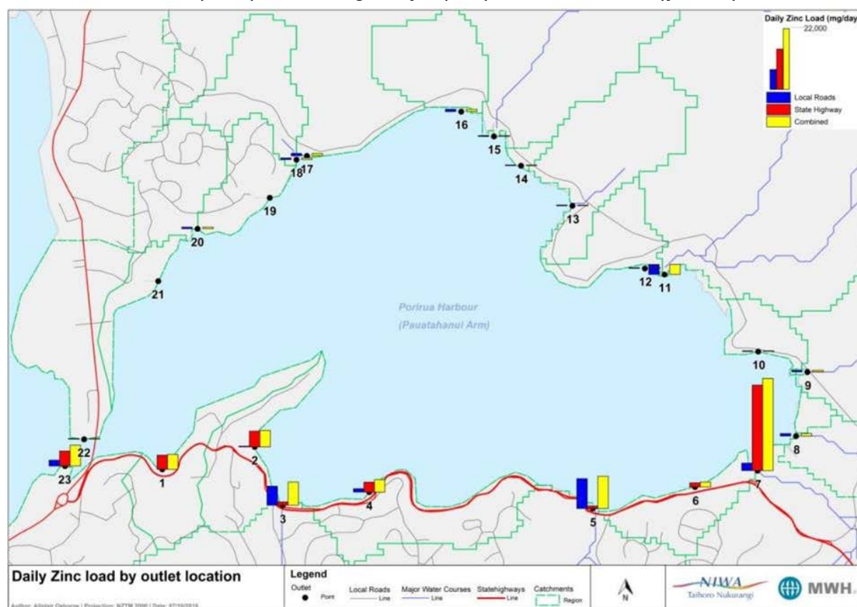
Figure 10 Relative contributions of zinc load to Pauatahanui Inlet from local roads (blue), state highways (red) and combined (yellow)
