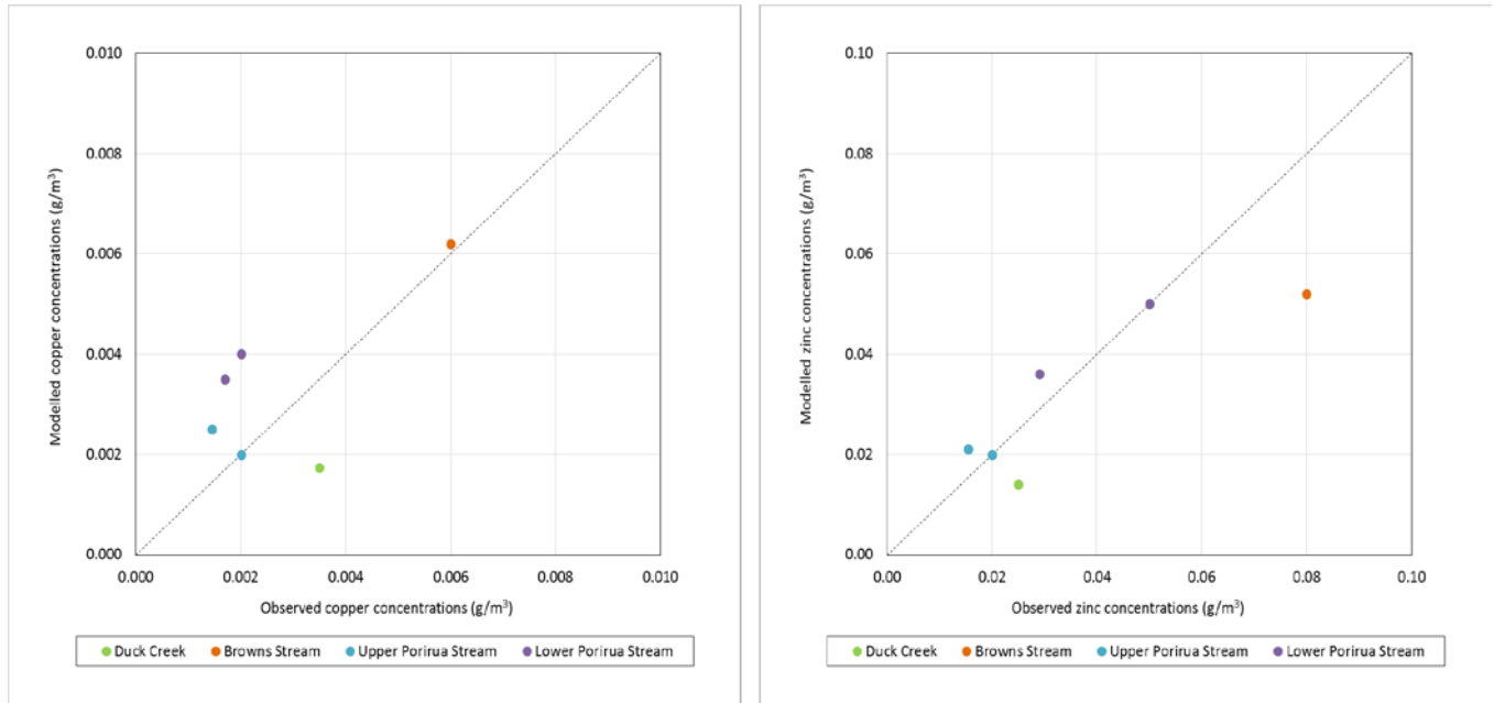
Figure 8 Total copper (left) and total zinc (right) measured in samples from stream reaches in the case study area, compared with modelled concentrations
